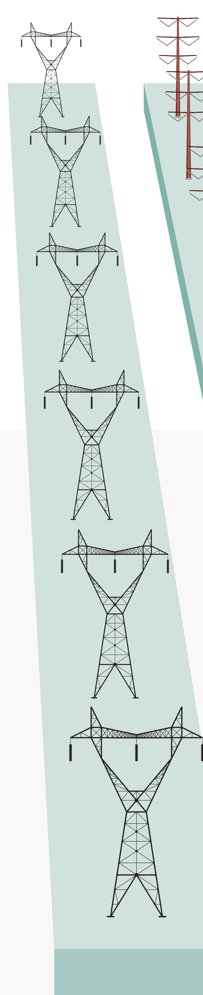
765 kV ONE SINGLE CIRCUIT TOWER (250 ft of total right-of-way)
